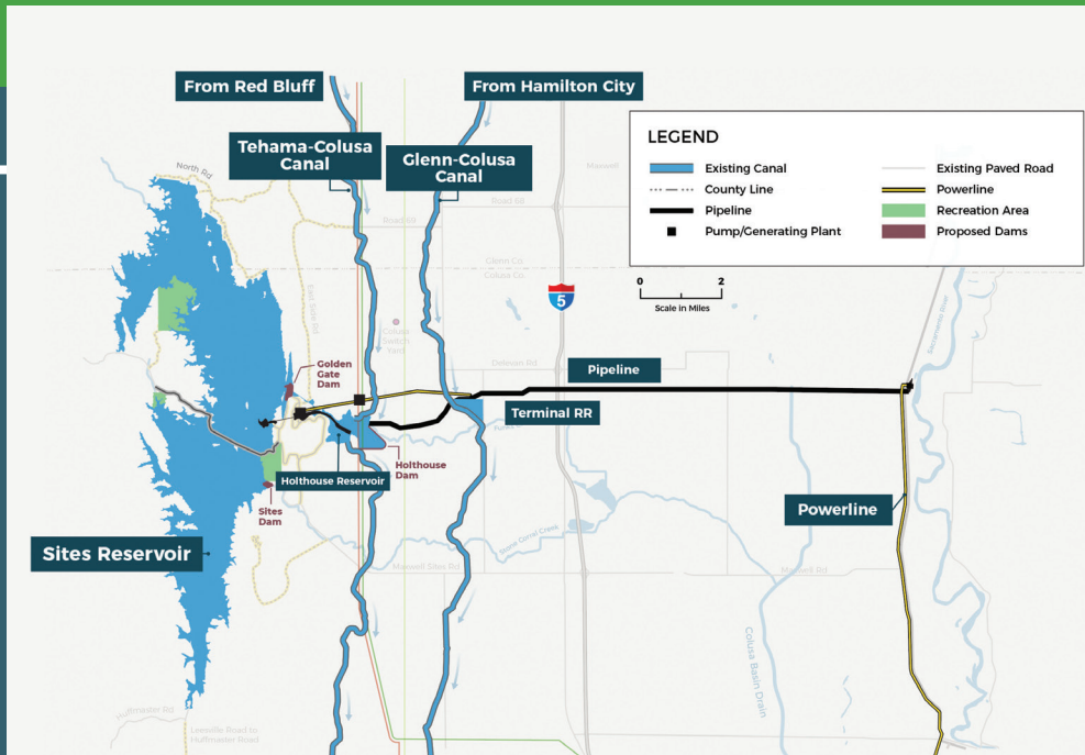
Located in rural Glenn and Colusa Counties, 10 miles west of the town of Maxwell, the Sites Reservoir would be a 1.8 million acre-foot off-stream storage facility.
