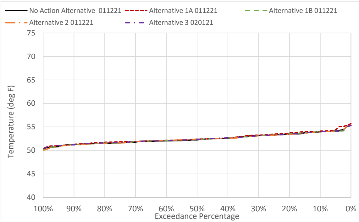
Figure 6D2-3-2. GCID Main Canal Water Temperature in November
