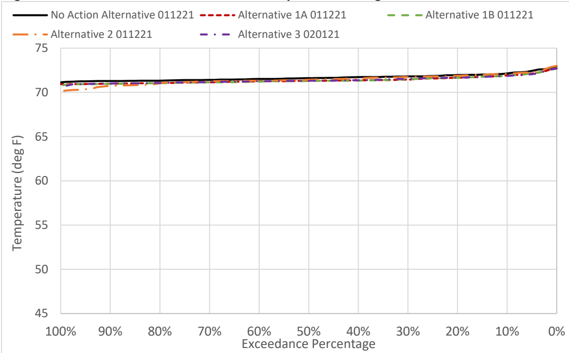
Figure 6D2-7-11. Sacramento River Water Temperature in August
