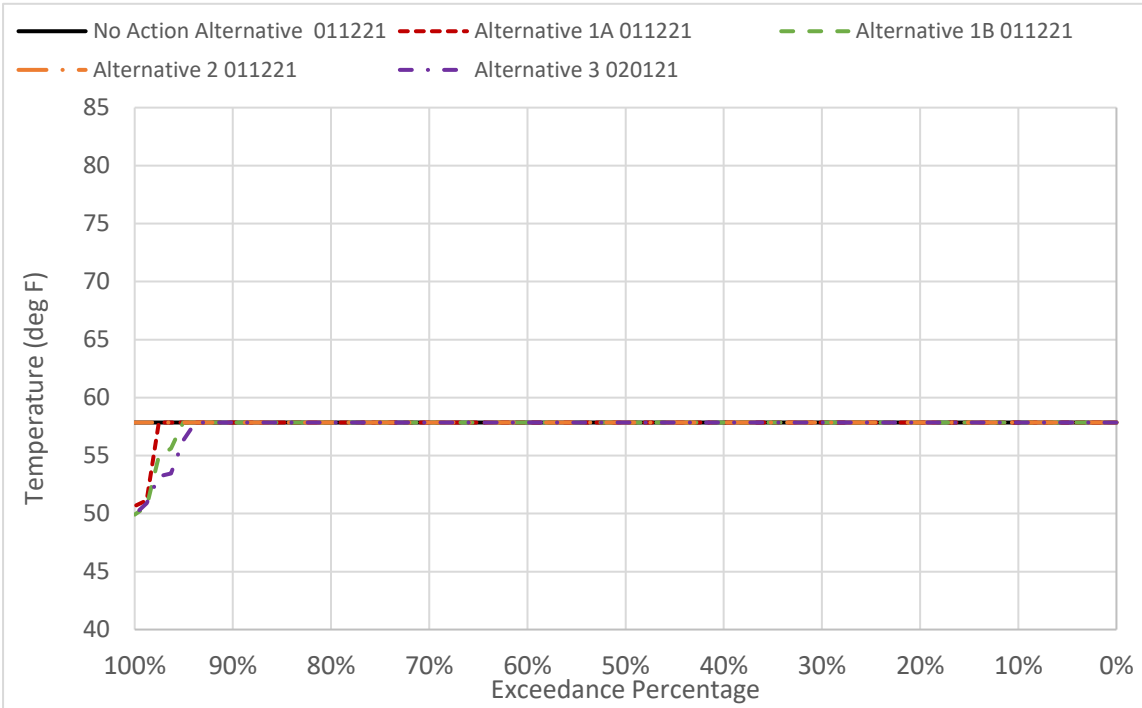
Figure 6D2-5-6. CBD Water Temperature in March
