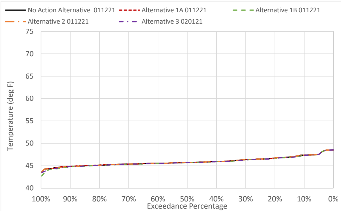
Figure 6D2-3-4. GCID Main Canal Water Temperature in January
