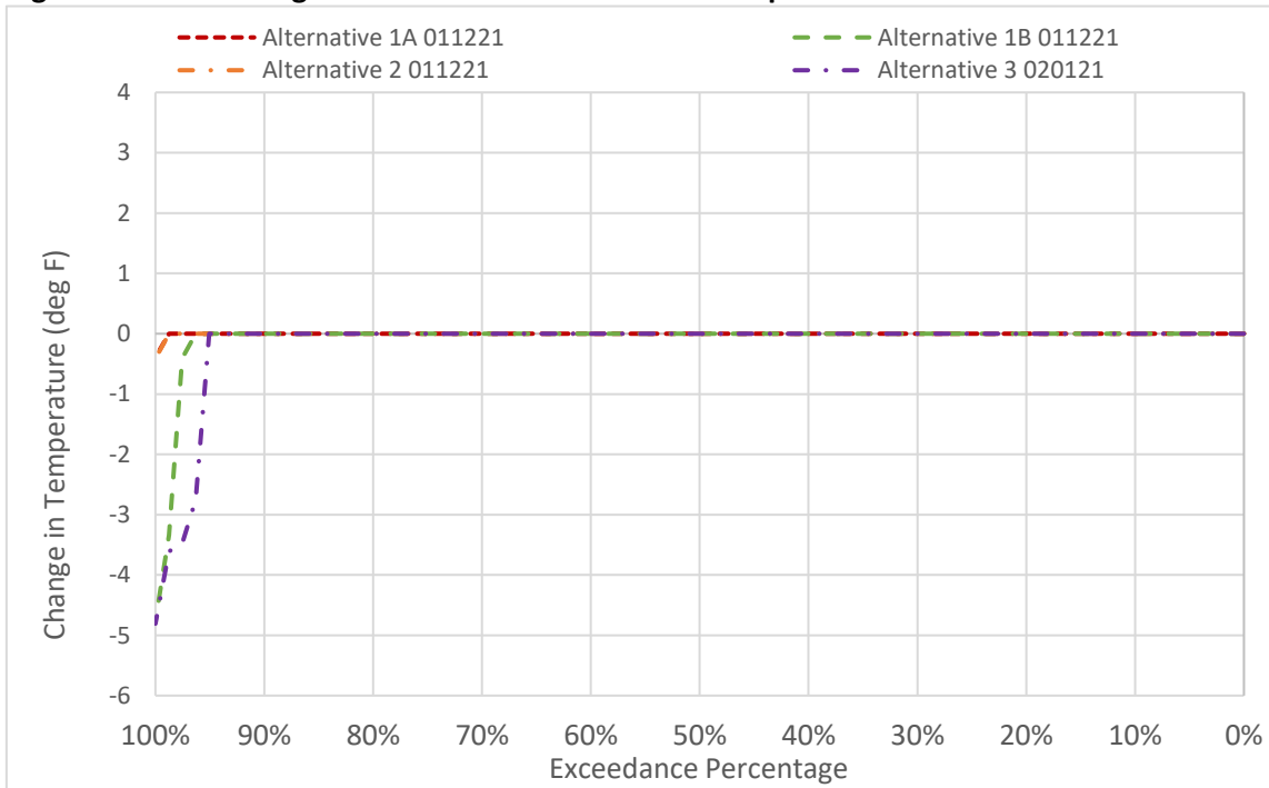
Figure 6D2-4-6. Changes to GCID Main Canal Water Temperature in March
