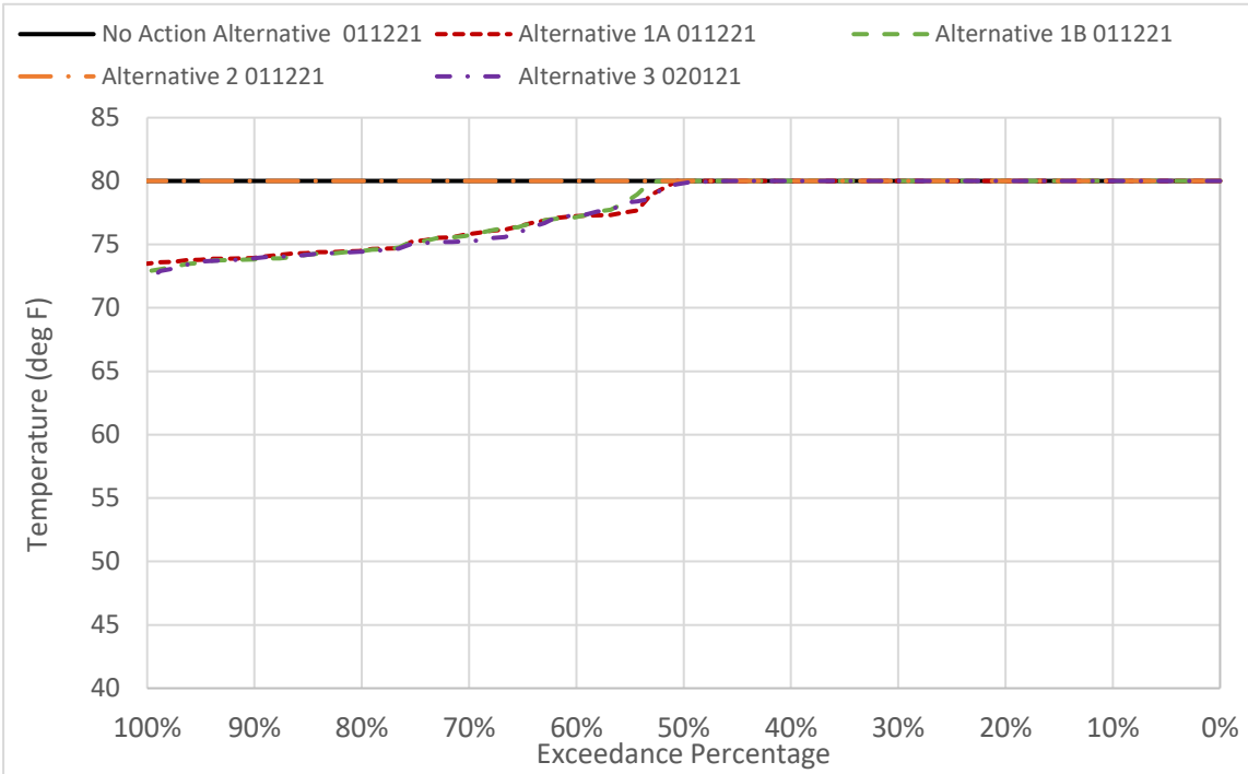
Figure 6D2-5-10. CBD Water Temperature in July
