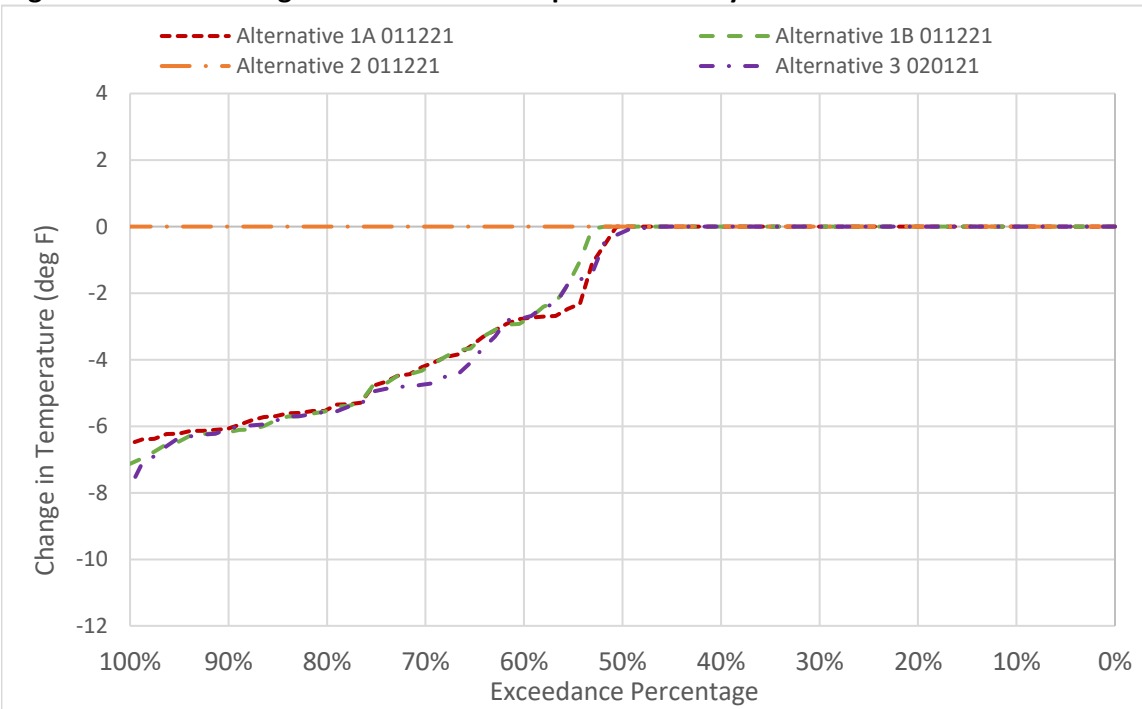
Figure 6D2-6-10. Changes to CBD Water Temperature in July
