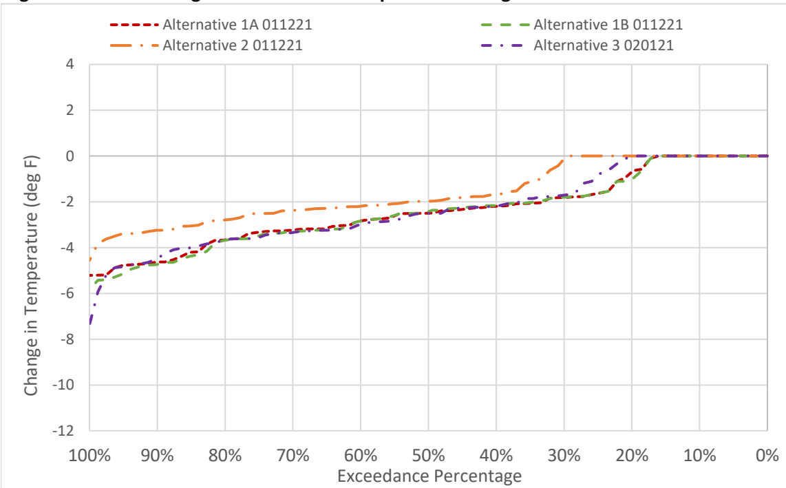
Figure 6D2-6-11. Changes to CBD Water Temperature in August
