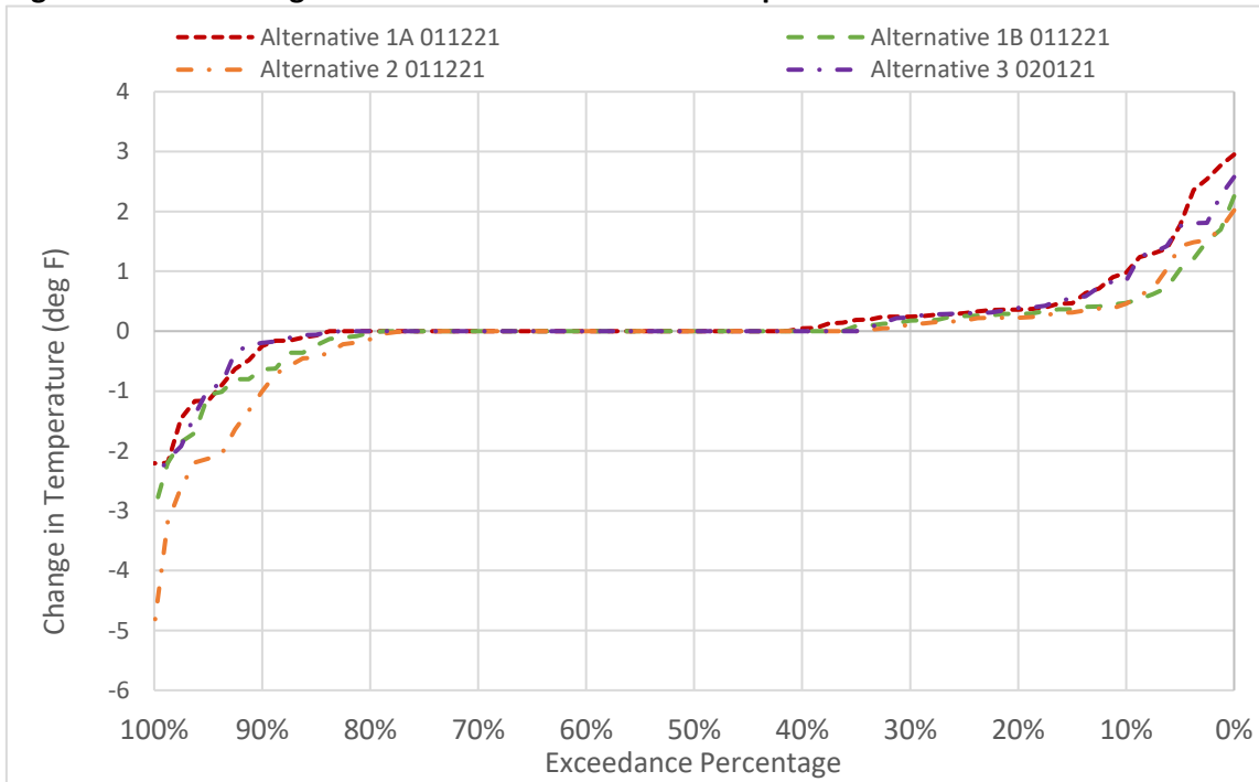
Figure 6D2-4-1. Changes to GCID Main Canal Water Temperature in October
