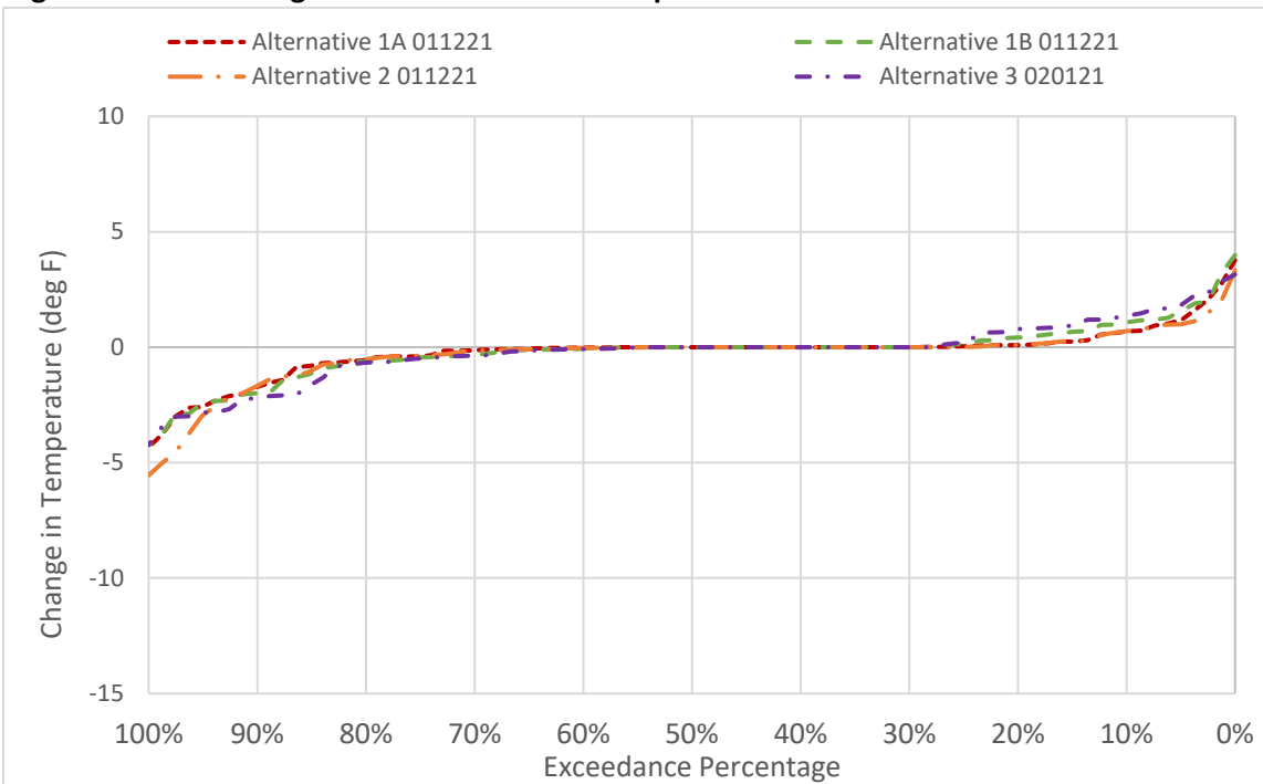
Figure 6D2-2-9. Changes to TC Canal Water Temperature in June
