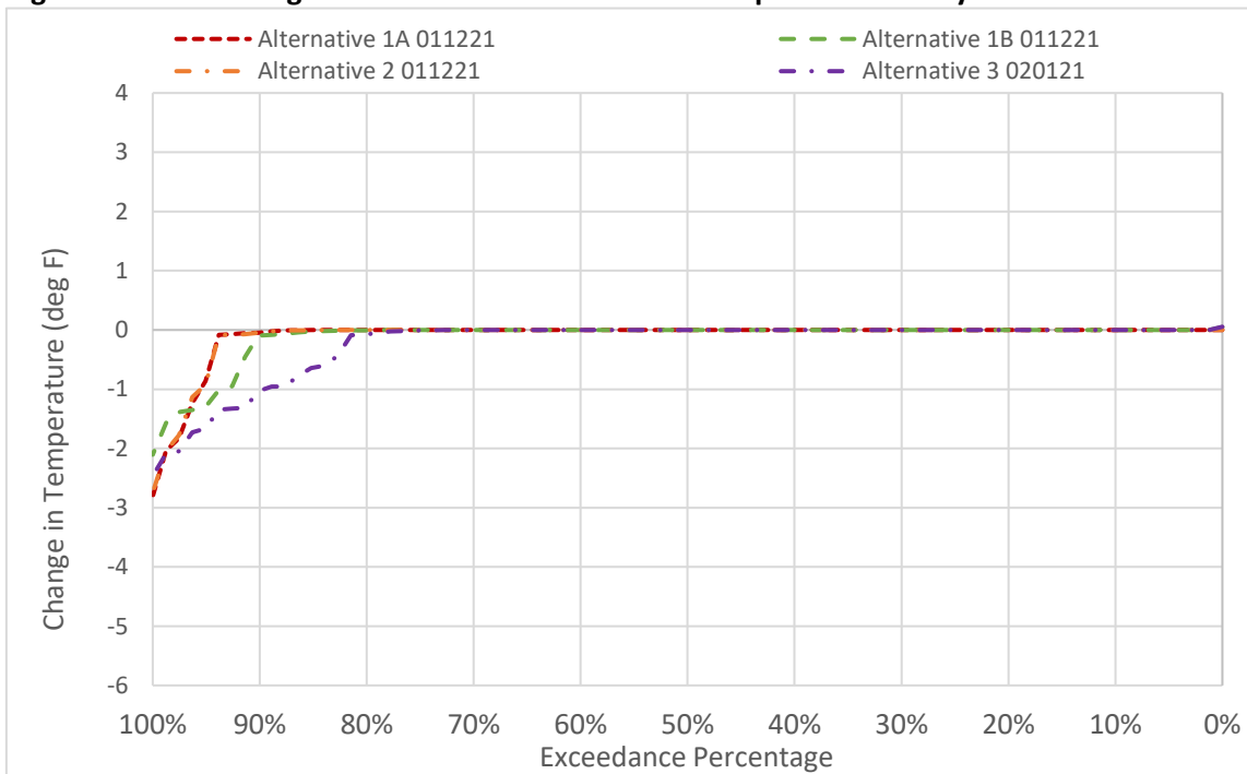
Figure 6D2-4-8. Changes to GCID Main Canal Water Temperature in May
