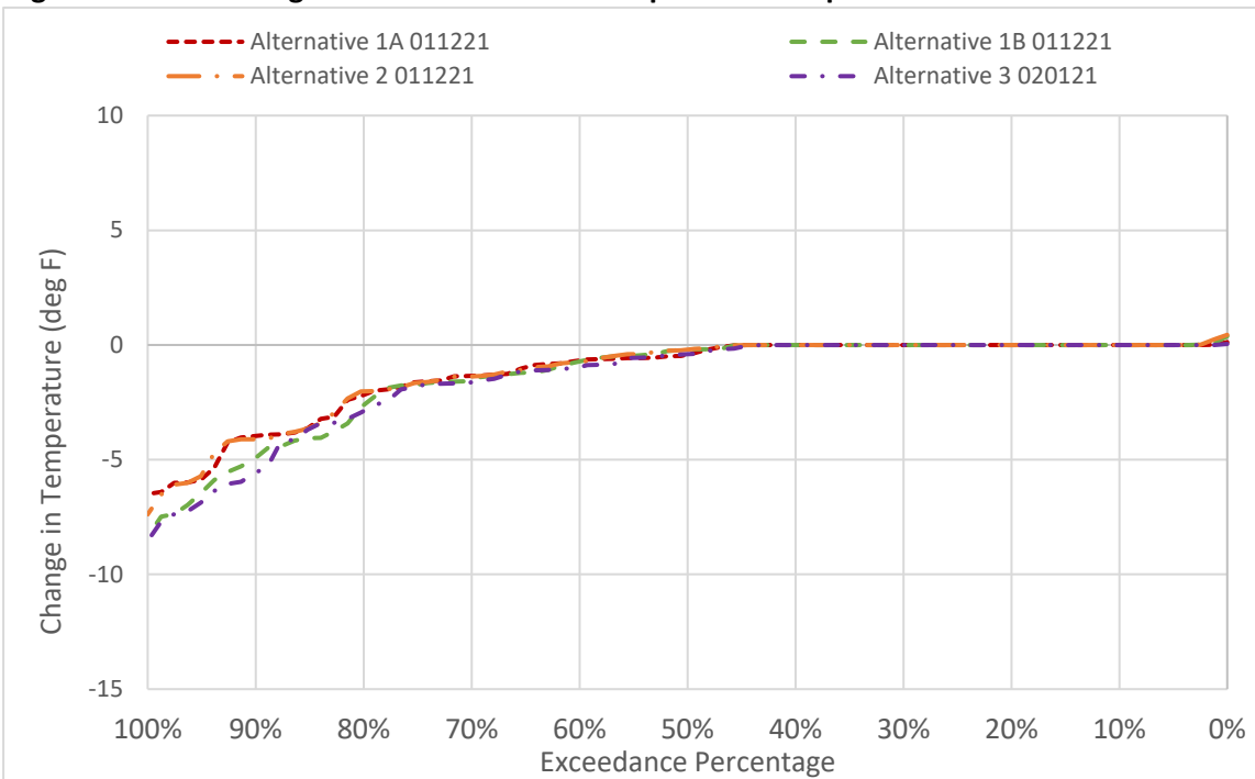
Figure 6D2-2-7. Changes to TC Canal Water Temperature in April
