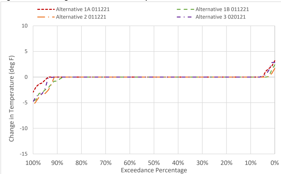
Figure 6D2-2-3. Changes to TC Canal Water Temperature in December
