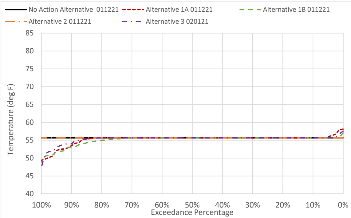
Figure 6D2-5-2. CBD Water Temperature in November
