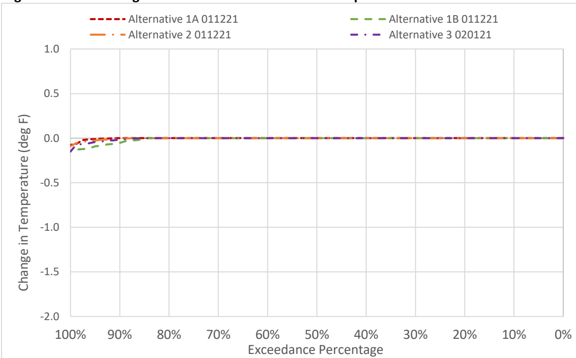
Figure 6D2-8-3. Changes to Sacramento River Water Temperature in December
