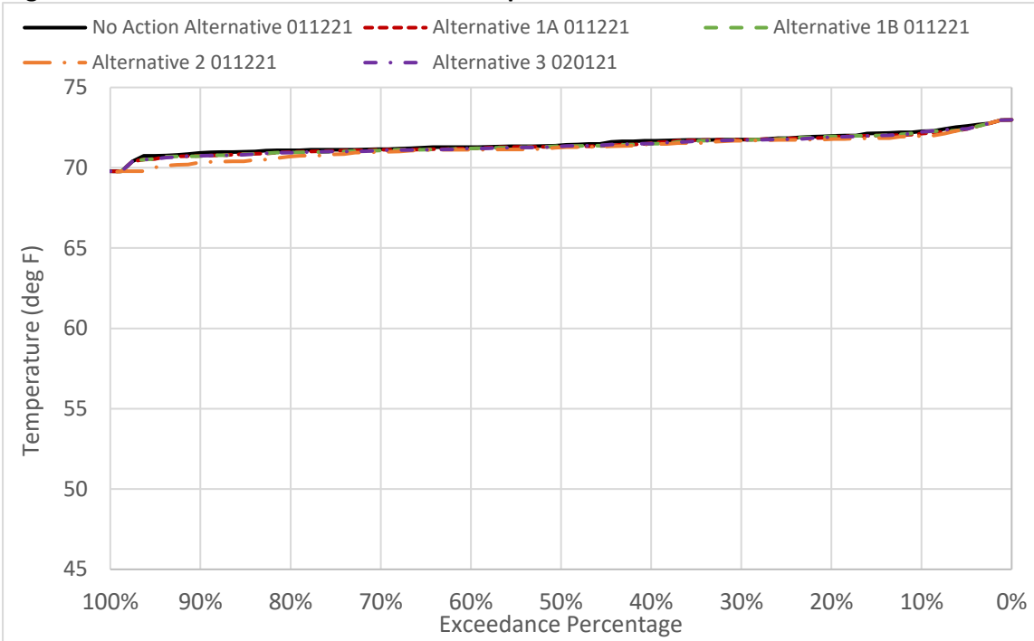
Figure 6D2-7-9. Sacramento River Water Temperature in June
