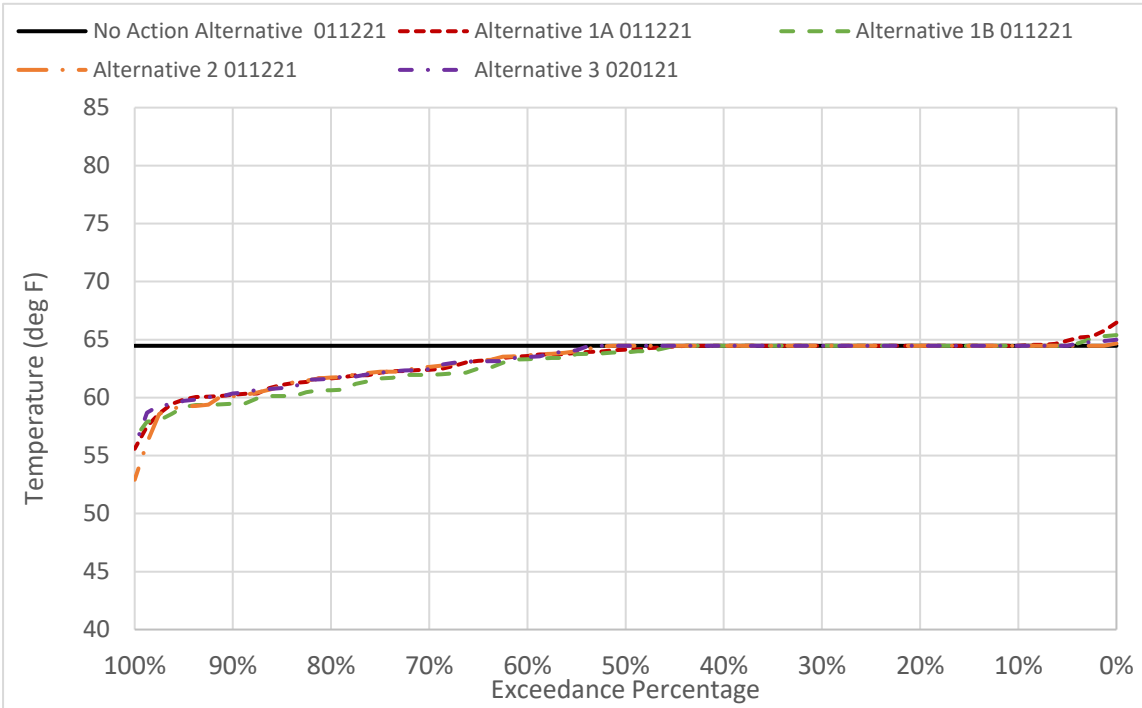
Figure 6D2-5-1. CBD Water Temperature in October
