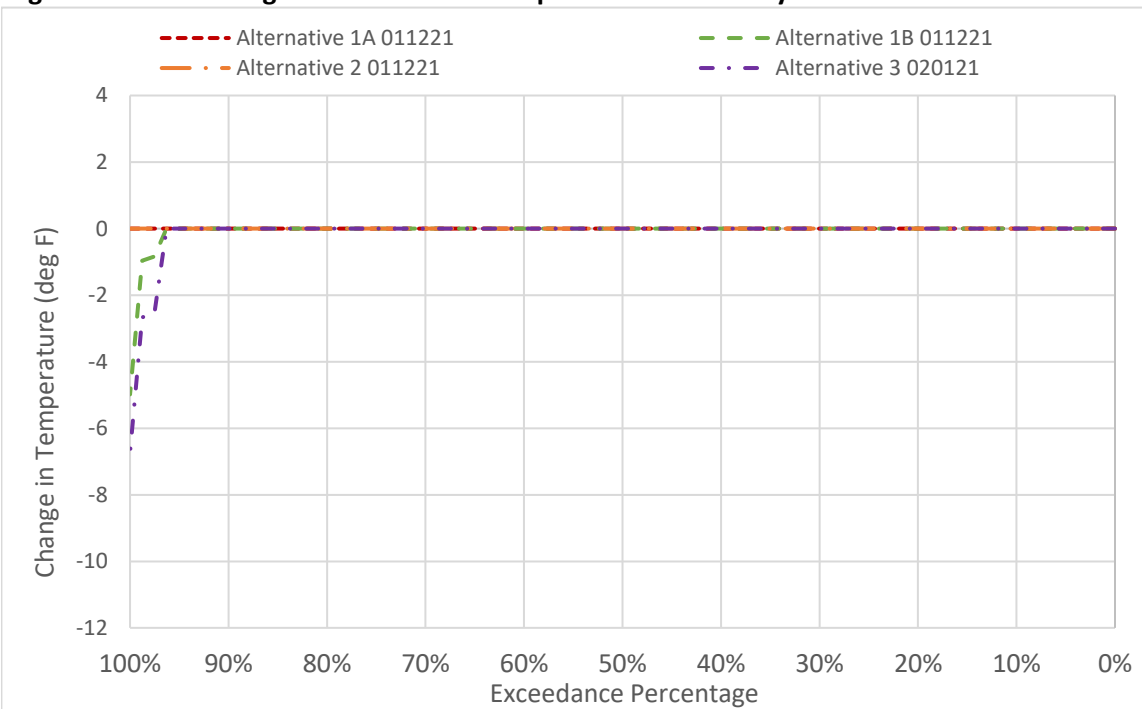
Figure 6D2-6-5. Changes to CBD Water Temperature in February
