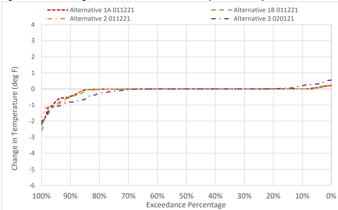
Figure 6D2-4-10. Changes to GCID Main Canal Water Temperature in July
