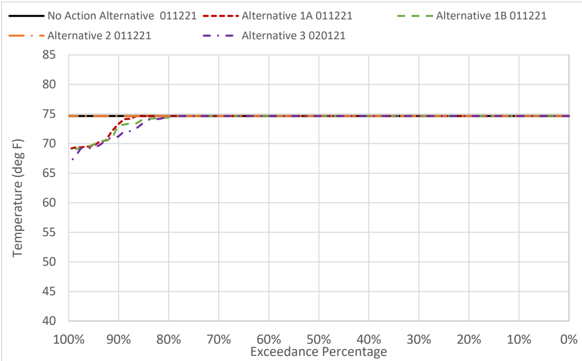
Figure 6D2-5-8. CBD Water Temperature in May
