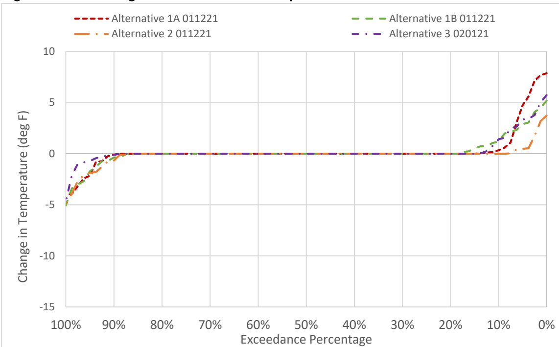
Figure 6D2-2-2. Changes to TC Canal Water Temperature in November
