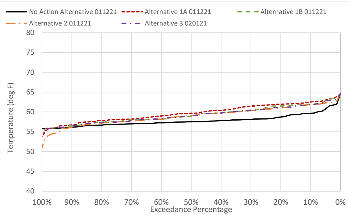
Figure 6D2-1-1. TC Canal Water Temperature in October
