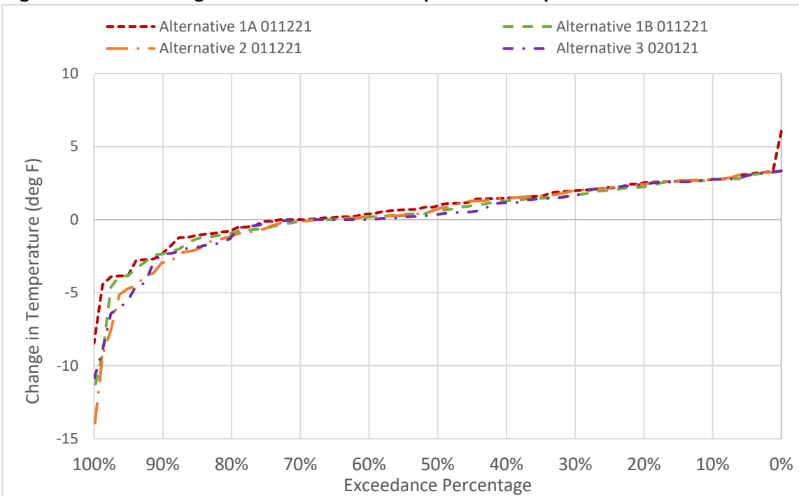
Figure 6D2-2-12. Changes to TC Canal Water Temperature in September
