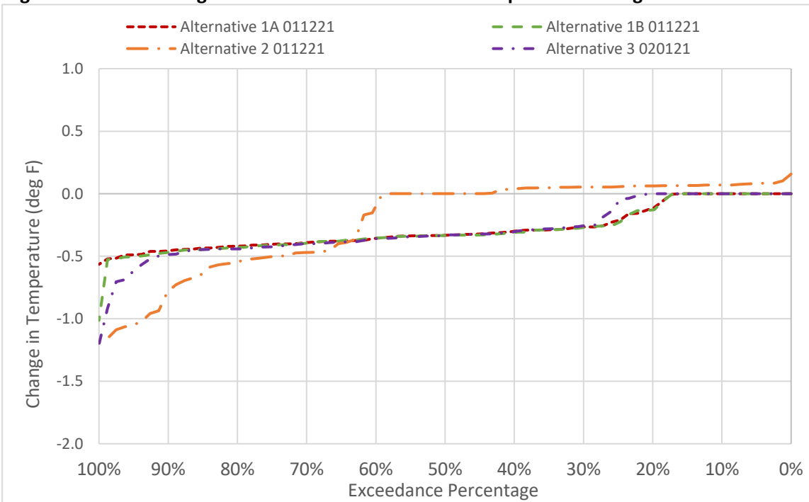
Figure 6D2-8-11. Changes to Sacramento River Water Temperature in August
