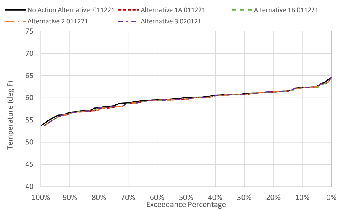
Figure 6D2-3-7. GCID Main Canal Water Temperature in April
