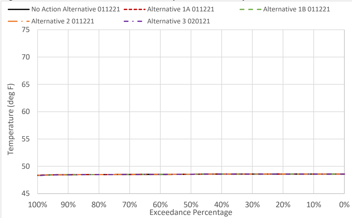
Figure 6D2-7-4. Sacramento River Water Temperature in January
