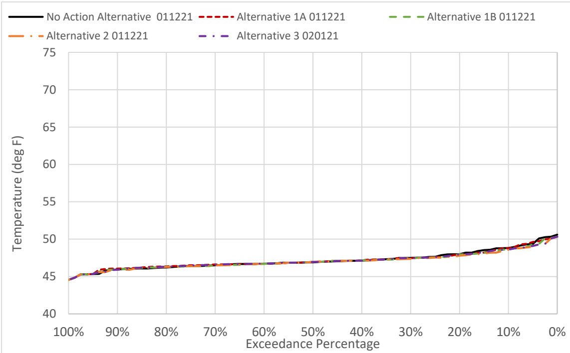
Figure 6D2-3-3. GCID Main Canal Water Temperature in December
