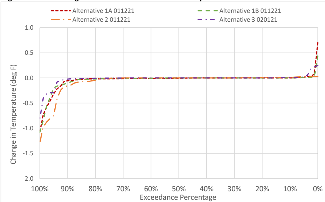
Figure 6D2-8-1. Changes to Sacramento River Water Temperature in October
