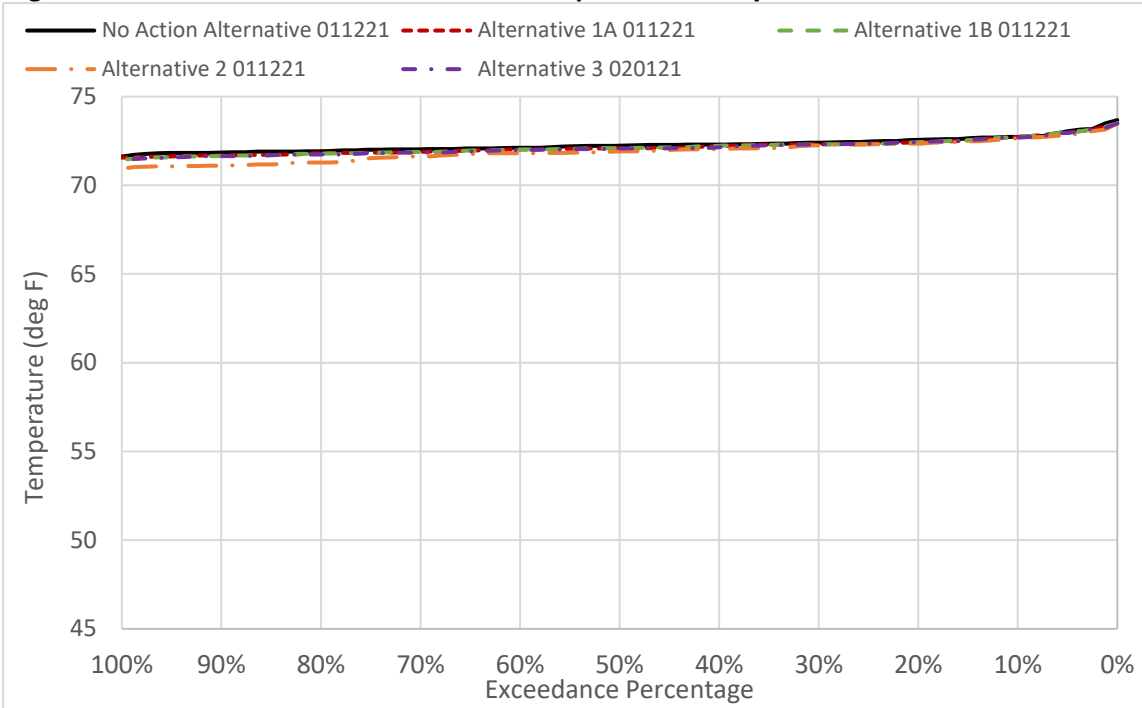
Figure 6D2-7-10. Sacramento River Water Temperature in July
