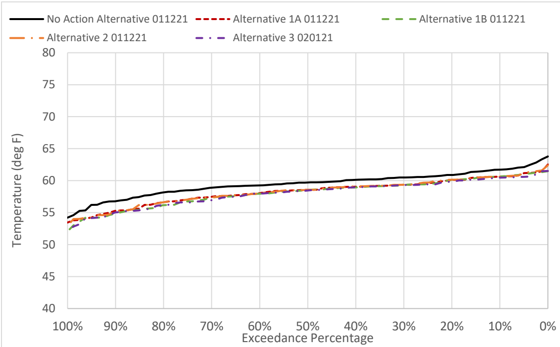
Figure 6D2-1-7. TC Canal Water Temperature in April
