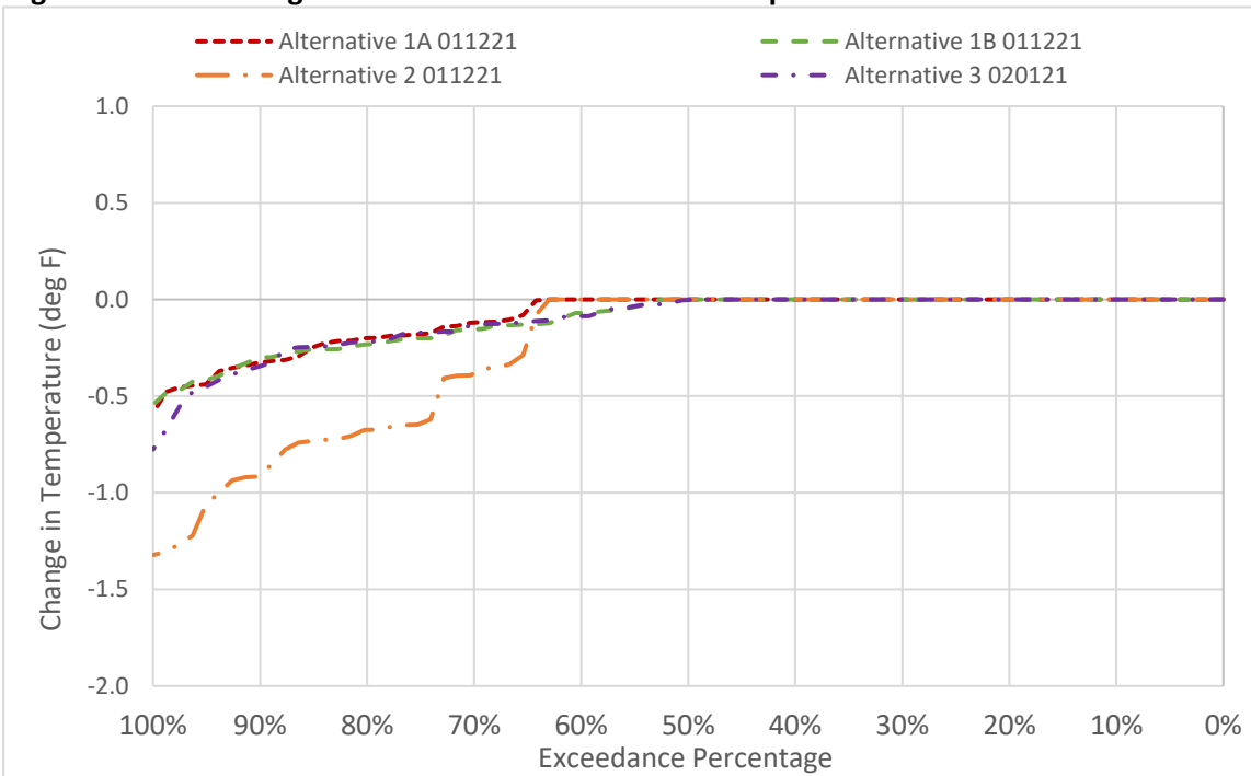
Figure 6D2-8-9. Changes to Sacramento River Water Temperature in June
