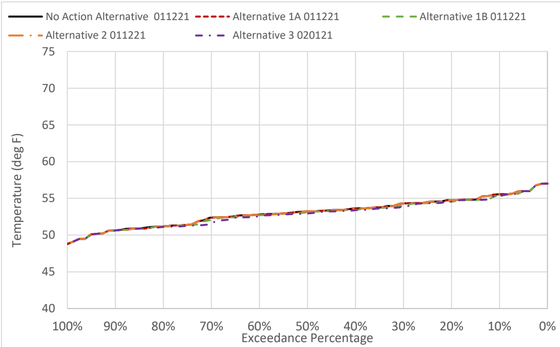
Figure 6D2-3-6. GCID Main Canal Water Temperature in March
