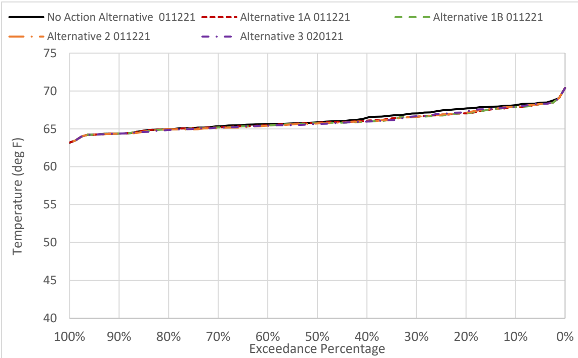
Figure 6D2-3-11. GCID Main Canal Water Temperature in August
