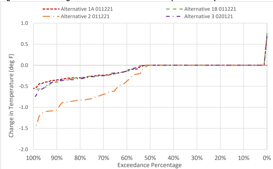
Figure 6D2-8-10. Changes to Sacramento River Water Temperature in July
