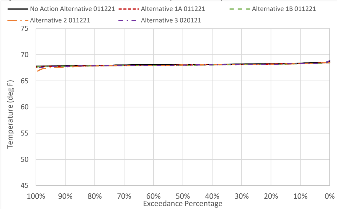
Figure 6D2-7-12. Sacramento River Water Temperature in September
