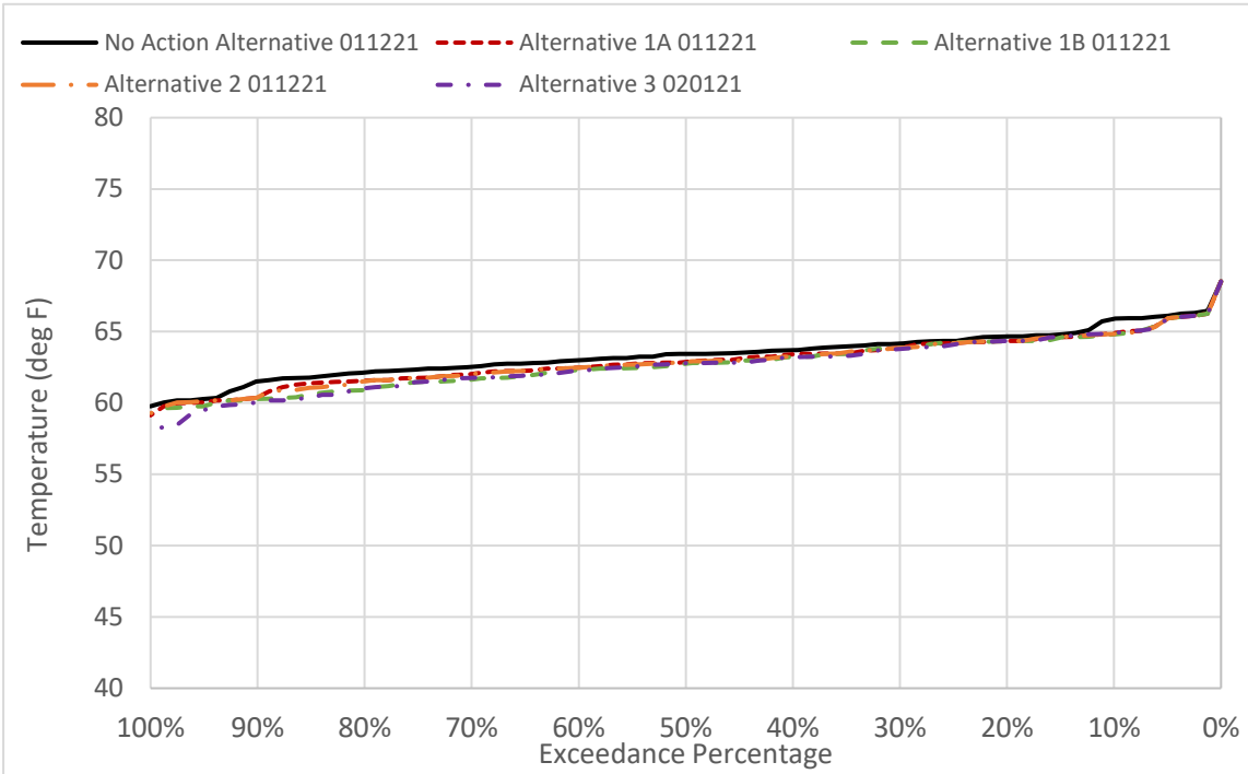
Figure 6D2-1-8. TC Canal Water Temperature in May
