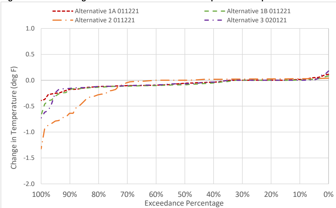
Figure 6D2-8-12. Changes to Sacramento River Water Temperature in September
