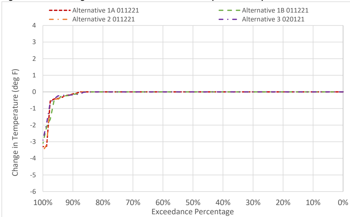
Figure 6D2-4-7. Changes to GCID Main Canal Water Temperature in April
