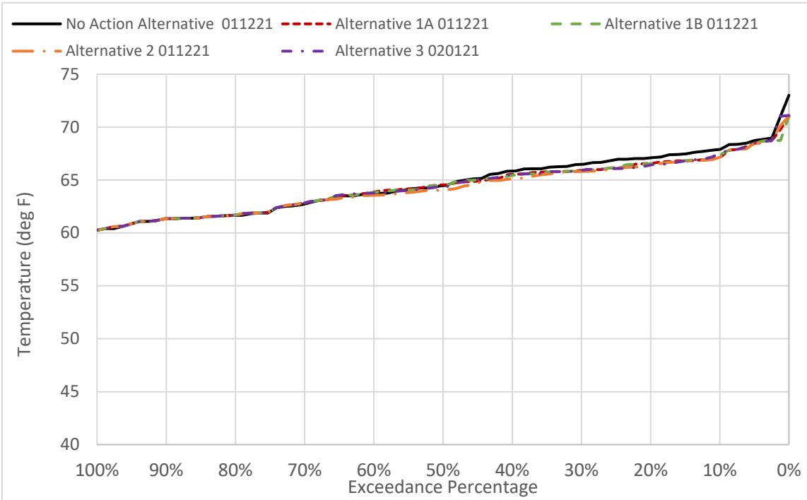
Figure 6D2-3-12. GCID Main Canal Water Temperature in September
