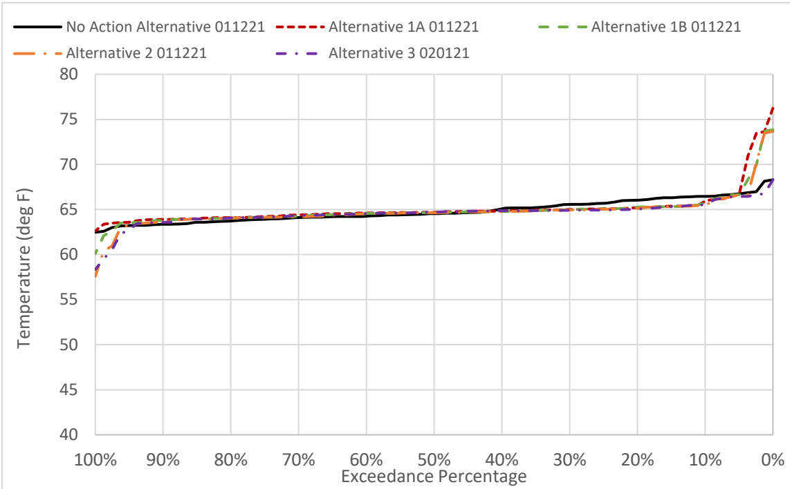
Figure 6D2-1-11. TC Canal Water Temperature in August
