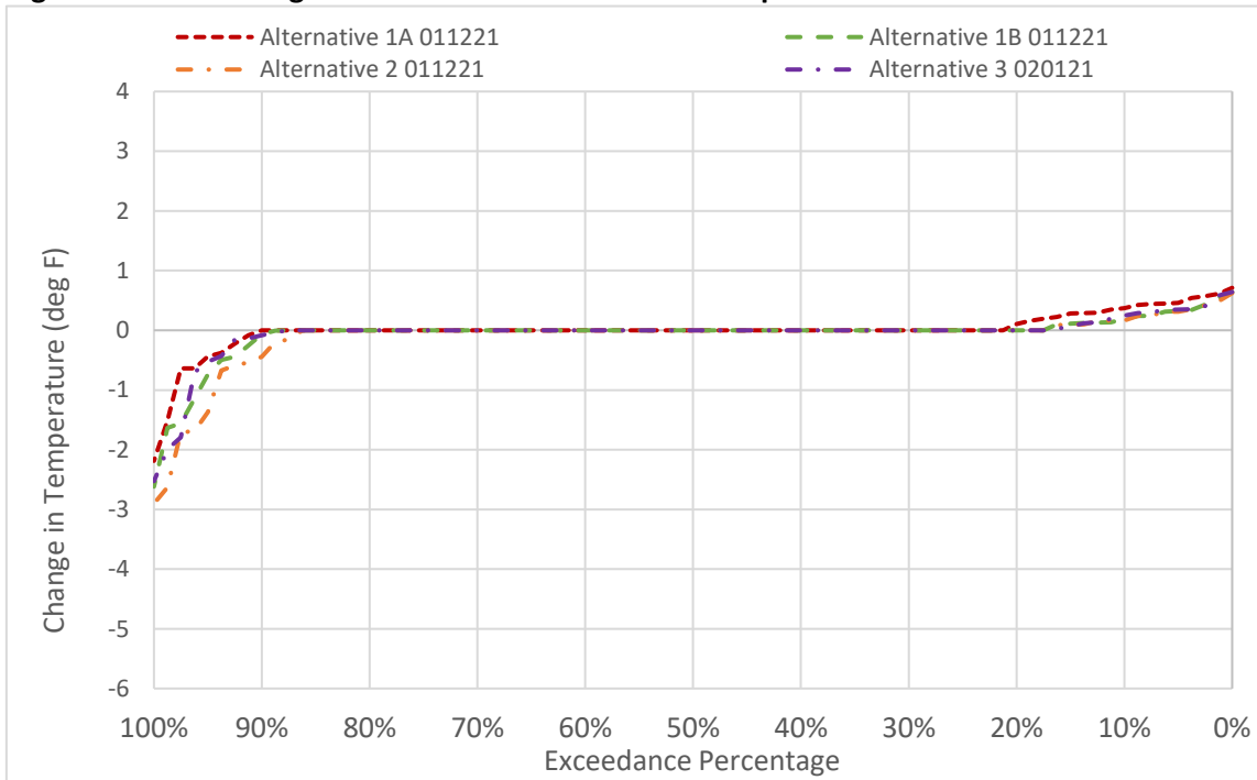
Figure 6D2-4-3. Changes to GCID Main Canal Water Temperature in December
