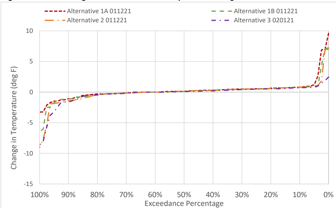
Figure 6D2-2-11. Changes to TC Canal Water Temperature in August
