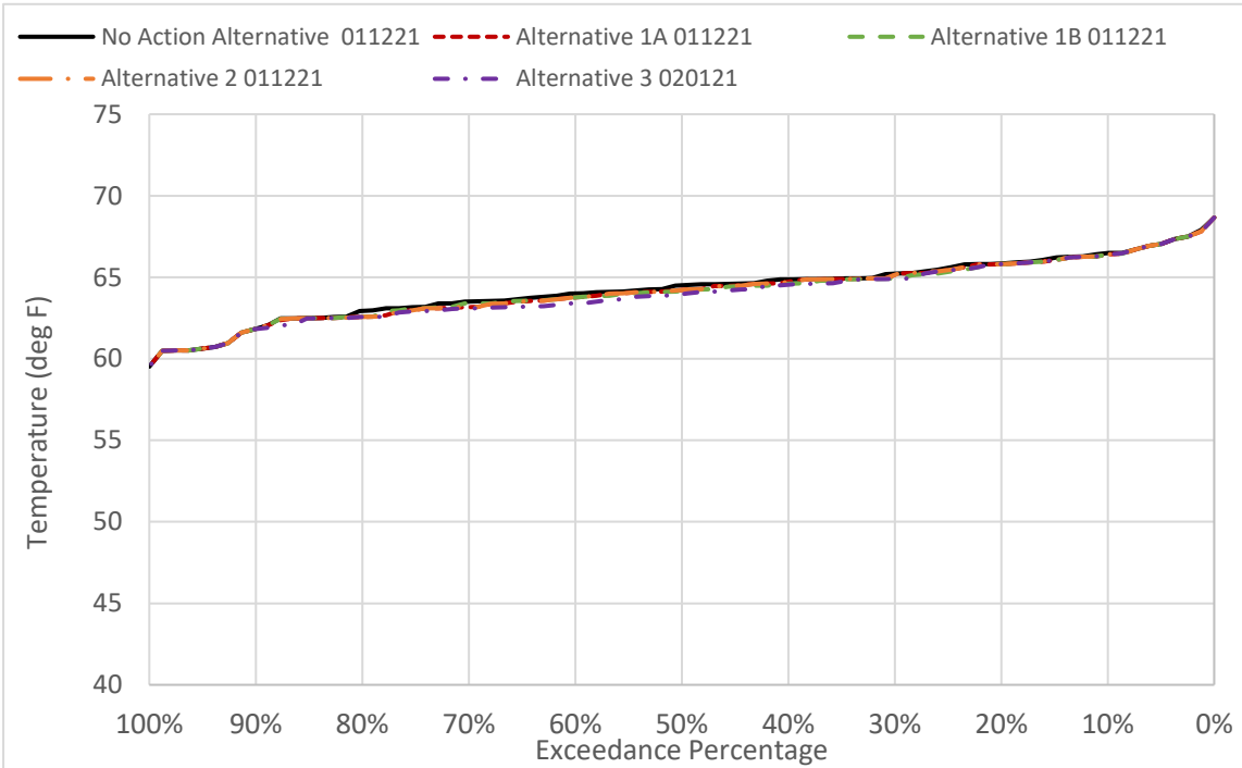
Figure 6D2-3-8. GCID Main Canal Water Temperature in May
