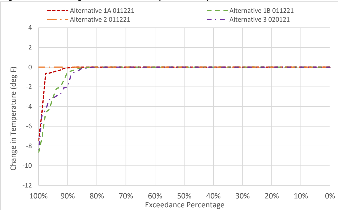
Figure 6D2-6-7. Changes to CBD Water Temperature in April
