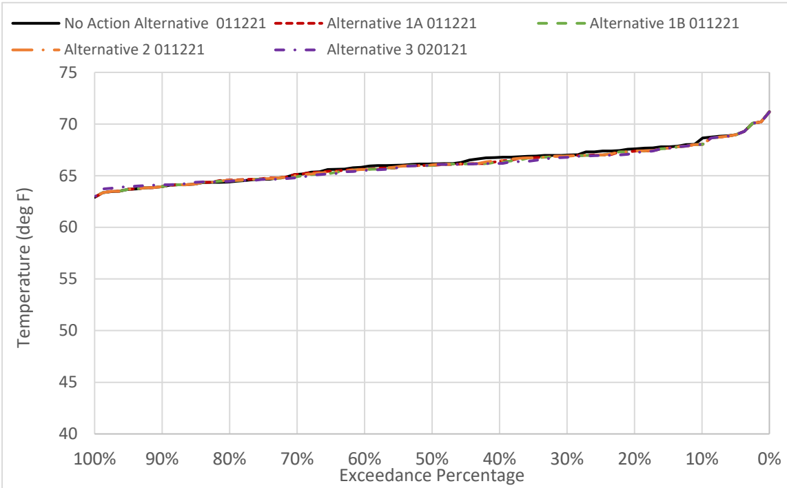
Figure 6D2-3-10. GCID Main Canal Water Temperature in July
