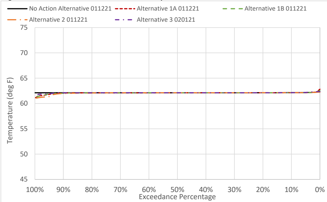
Figure 6D2-7-1. Sacramento River Water Temperature in October
