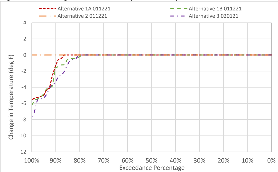
Figure 6D2-6-8. Changes to CBD Water Temperature in May
