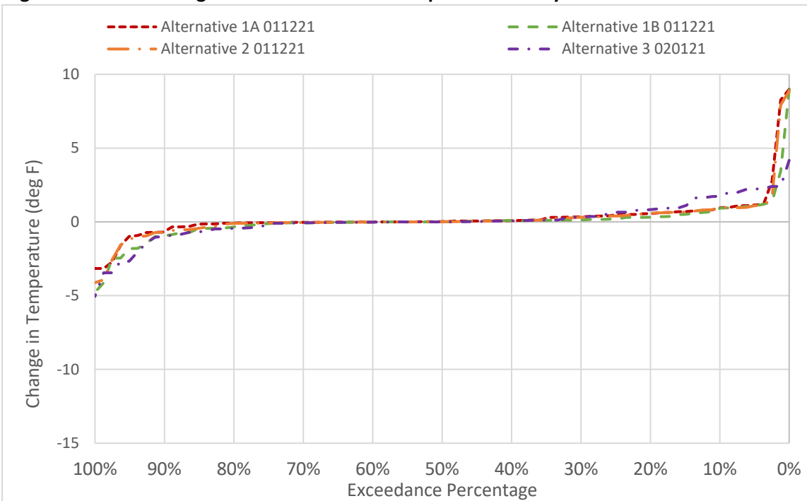
Figure 6D2-2-10. Changes to TC Canal Water Temperature in July
