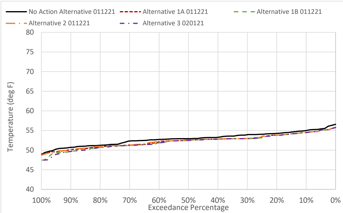
Figure 6D2-1-6. TC Canal Water Temperature in March
