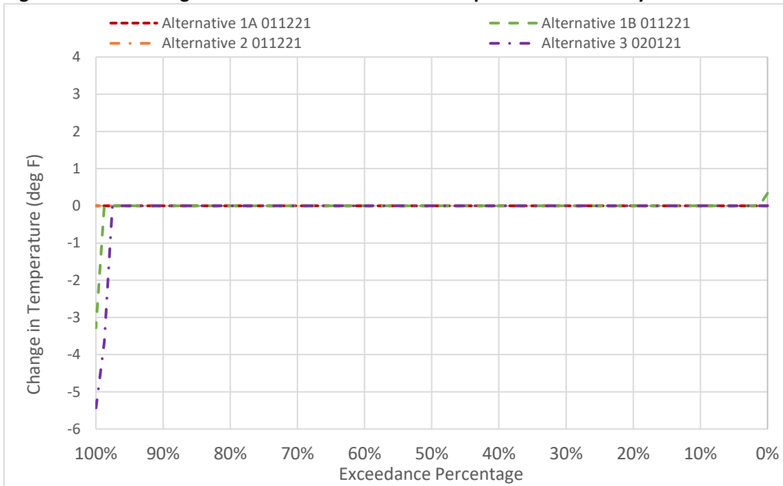
Figure 6D2-4-5. Changes to GCID Main Canal Water Temperature in February
