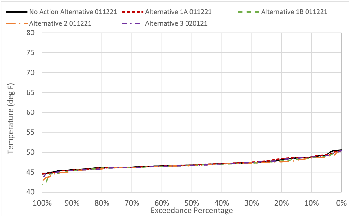
Figure 6D2-1-3. TC Canal Water Temperature in December
