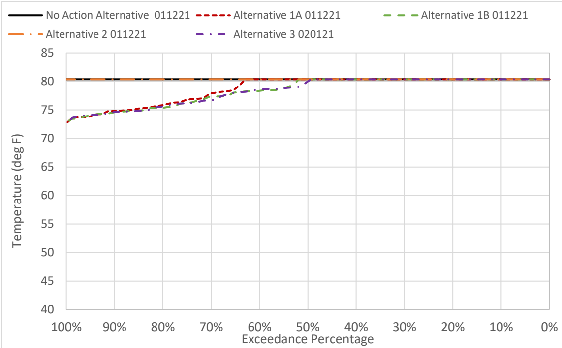
Figure 6D2-5-9. CBD Water Temperature in June
