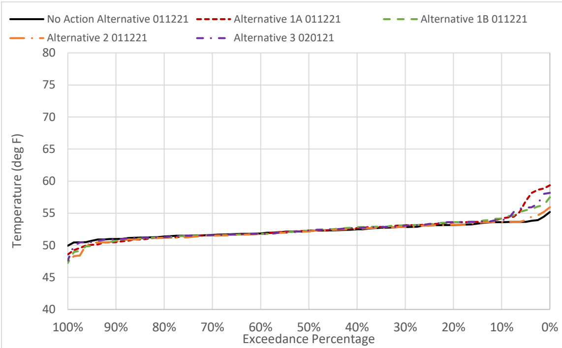
Figure 6D2-1-2. TC Canal Water Temperature in November
