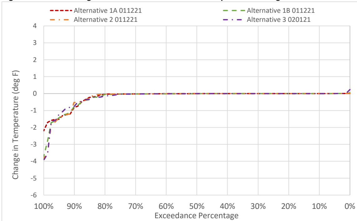
Figure 6D2-4-11. Changes to GCID Main Canal Water Temperature in August
