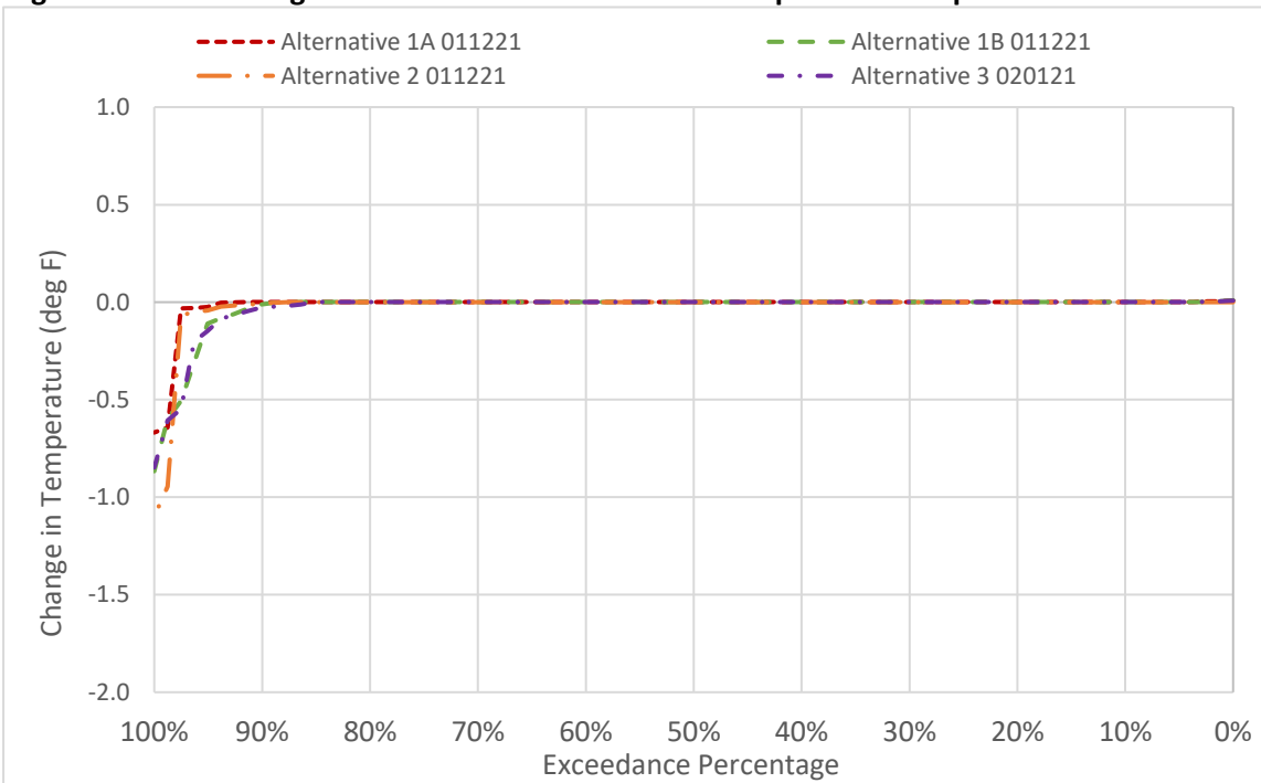
Figure 6D2-8-7. Changes to Sacramento River Water Temperature in April
