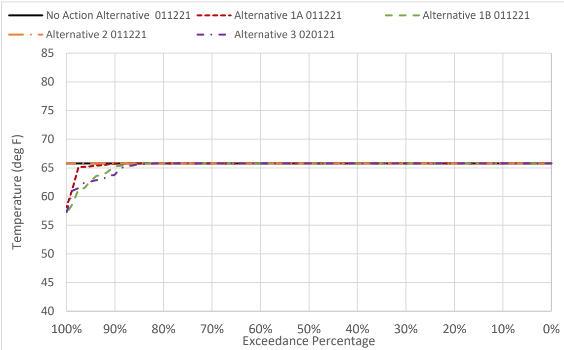
Figure 6D2-5-7. CBD Water Temperature in April
