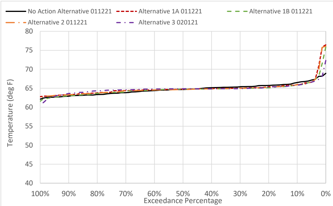
Figure 6D2-1-10. TC Canal Water Temperature in July
