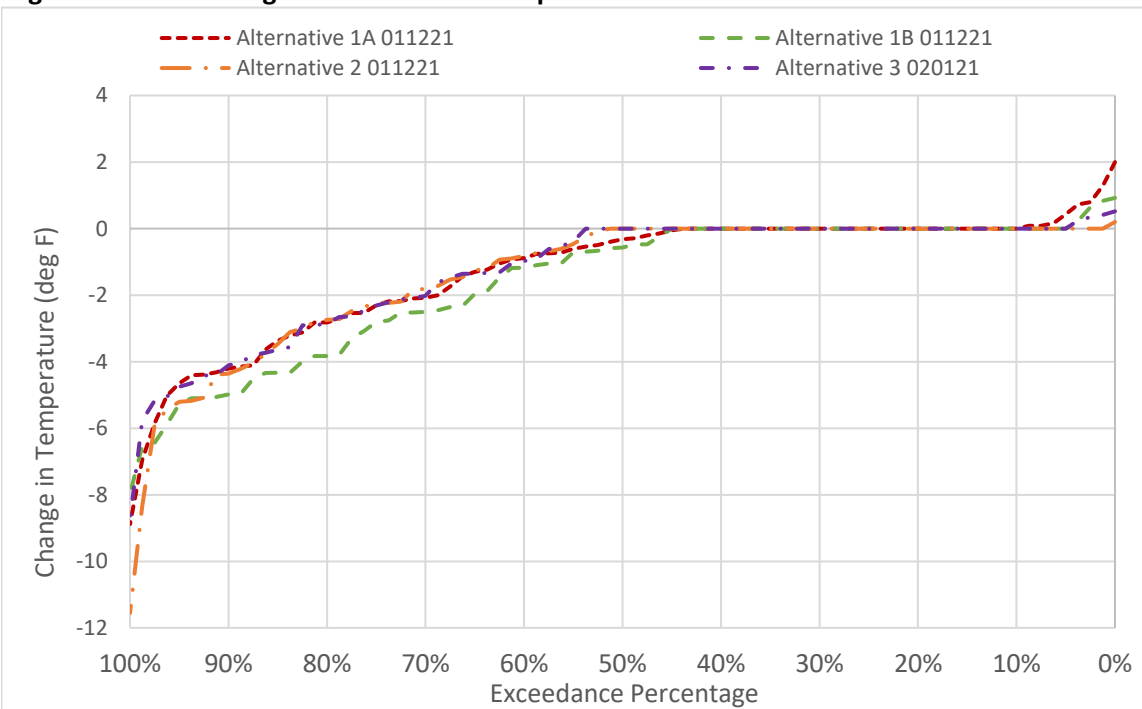
Figure 6D2-6-1. Changes to CBD Water Temperature in October
