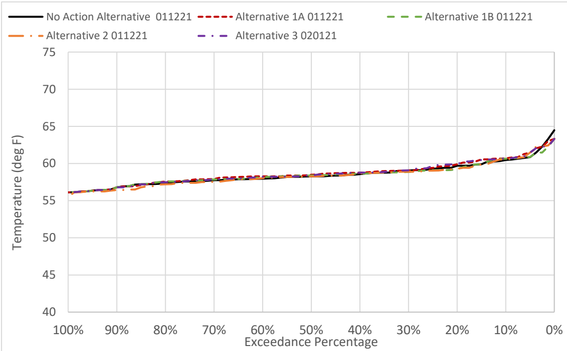
Figure 6D2-3-1. GCID Main Canal Water Temperature in October
