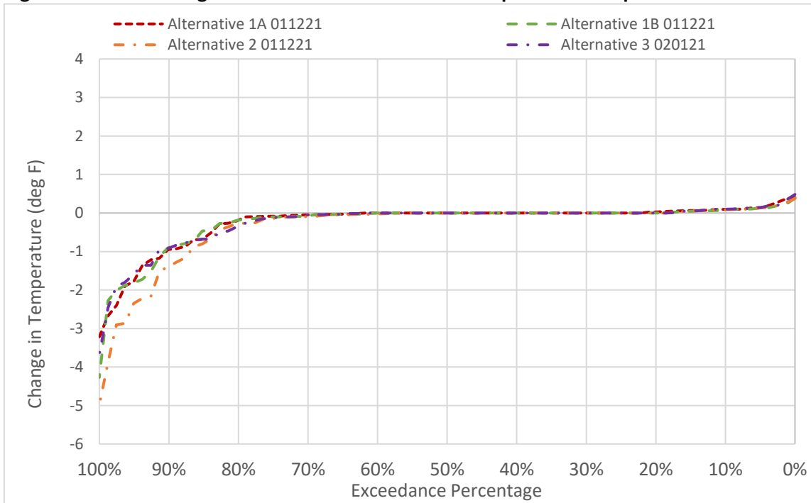
Figure 6D2-4-12. Changes to GCID Main Canal Water Temperature in September
