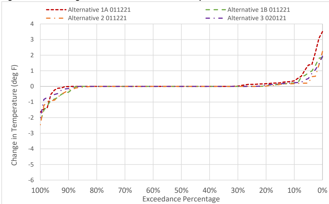
Figure 6D2-4-2. Changes to GCID Main Canal Water Temperature in November
