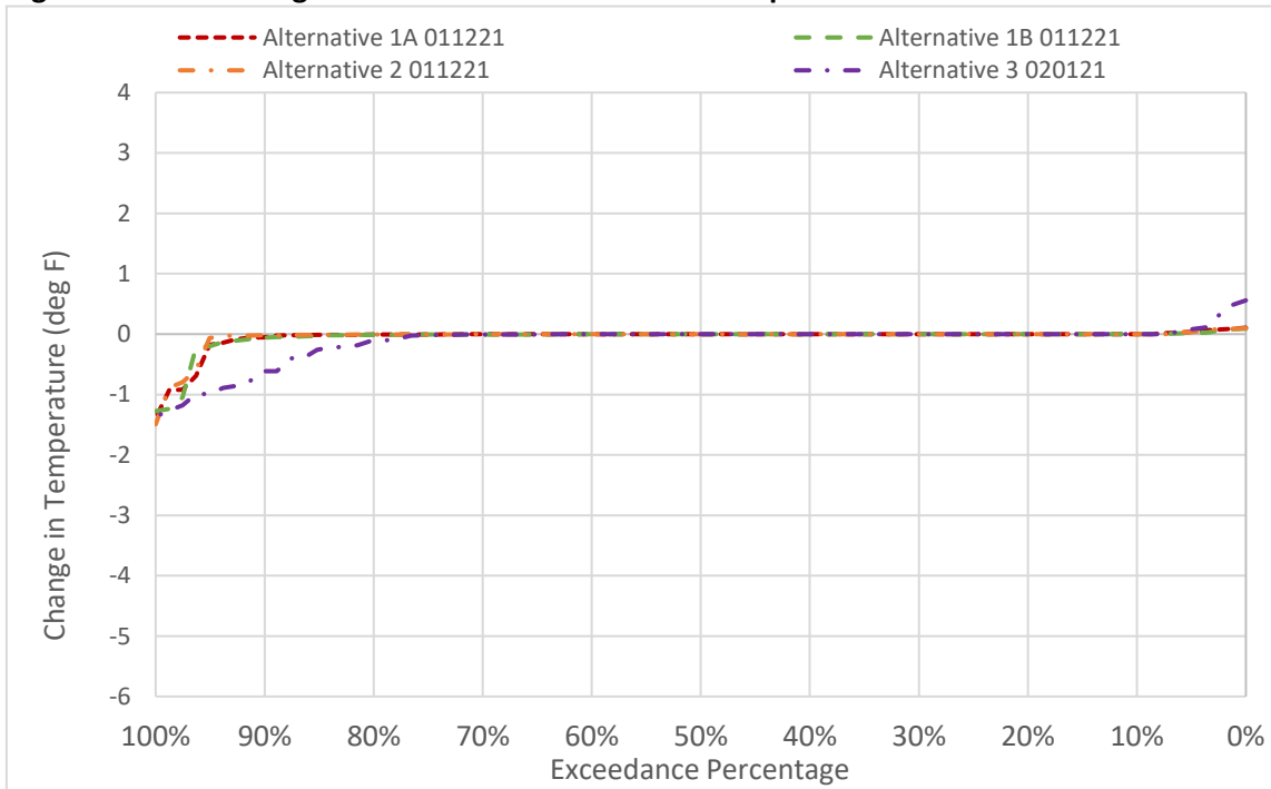
Figure 6D2-4-9. Changes to GCID Main Canal Water Temperature in June
