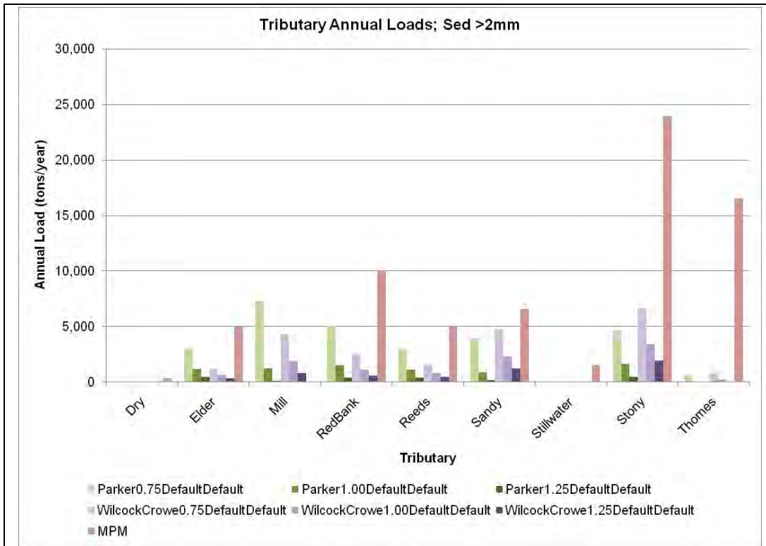
Figure 2-14. Tributary transport capacity sensitivity for last 9 alphabetically.
