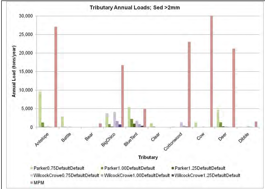
Figure 2-13. Tributary transport capacity sensitivity for first 10 alphabetically.
