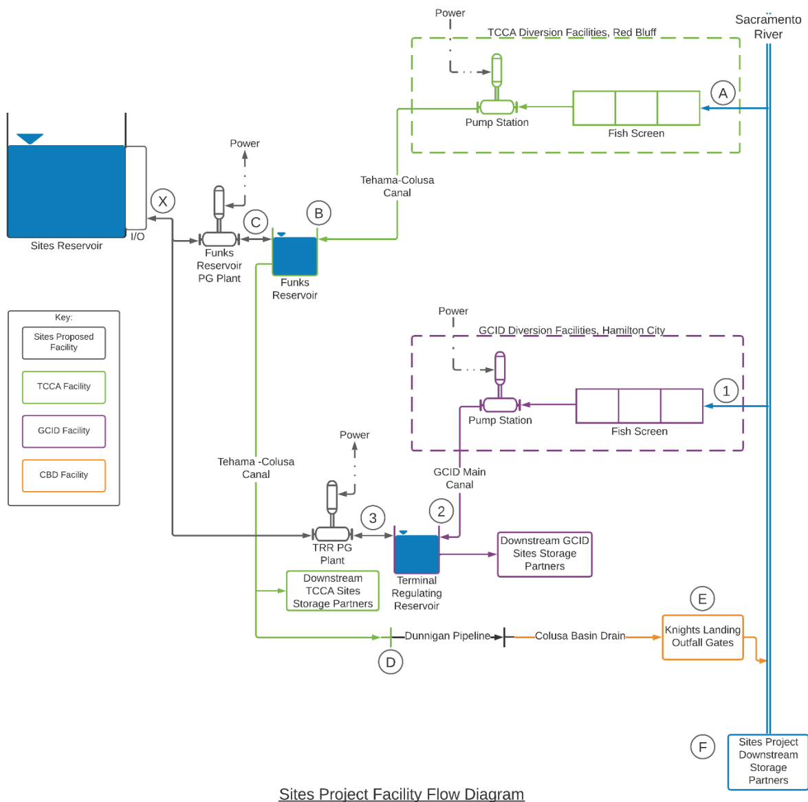
Figure 5-1. Sites Project facility flow diagram
