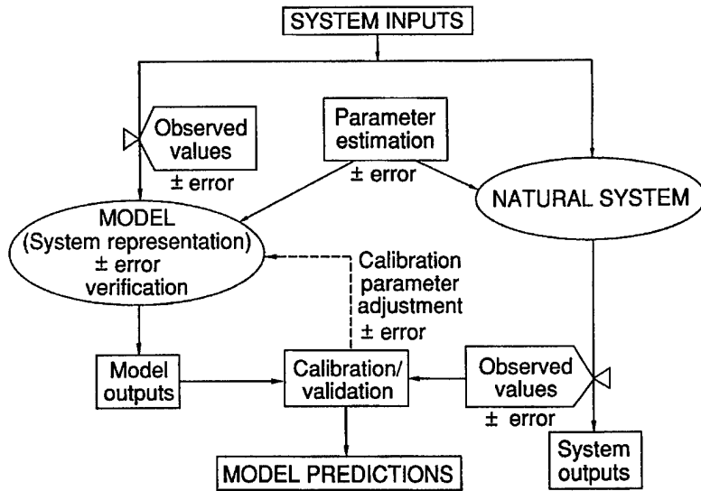
Fig. 5.1. Calibration process.
