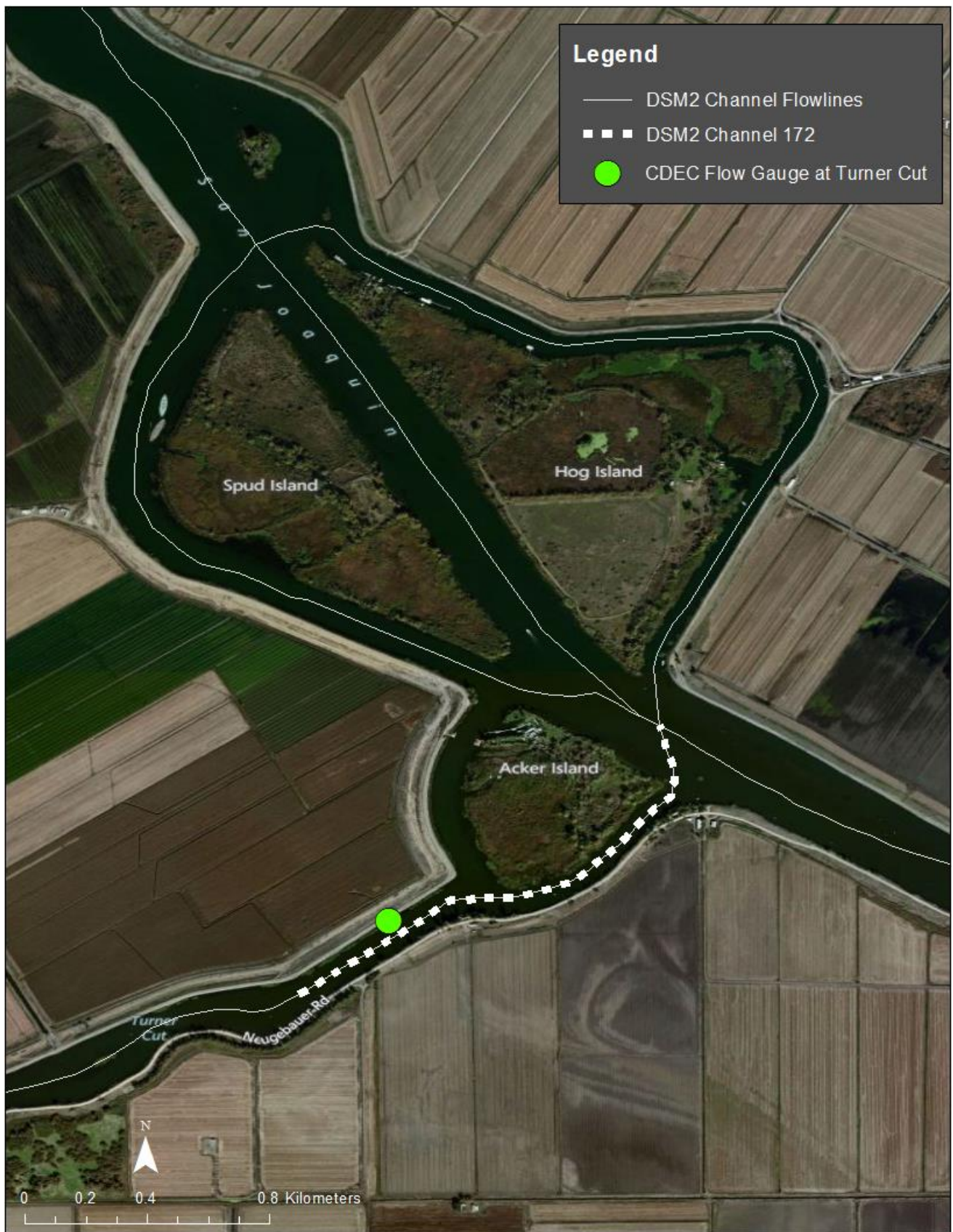
Figure 1-2 The location of DSM2 channel 172 and the gauging station at Turner Cut.
